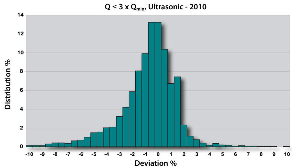
Fig. 6: 3 \times Q_{min} 2010, Kamstrup ultrasonic meters
