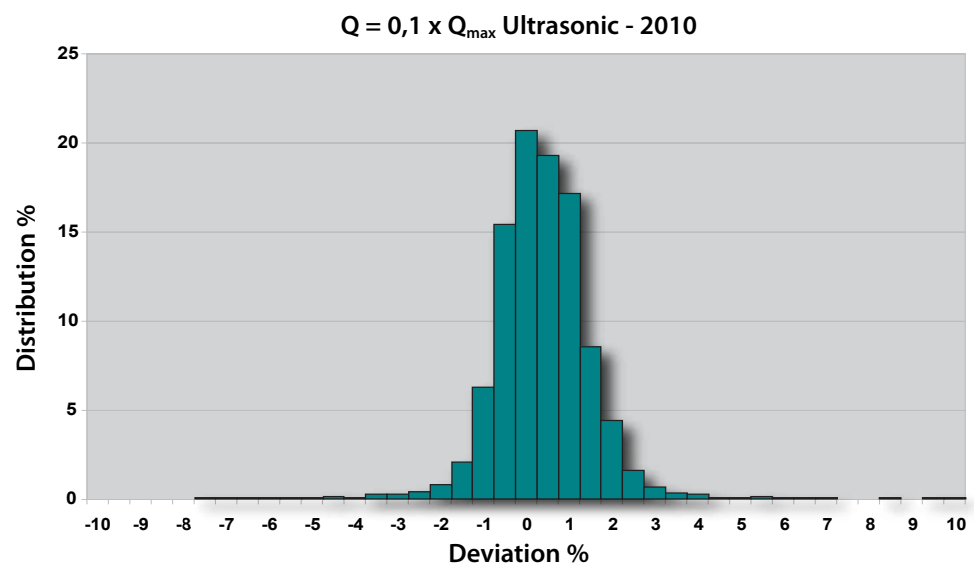
Fig. 5: 0,1 \times Q_{max} 2010, Kamstrup ultrasonic meters
